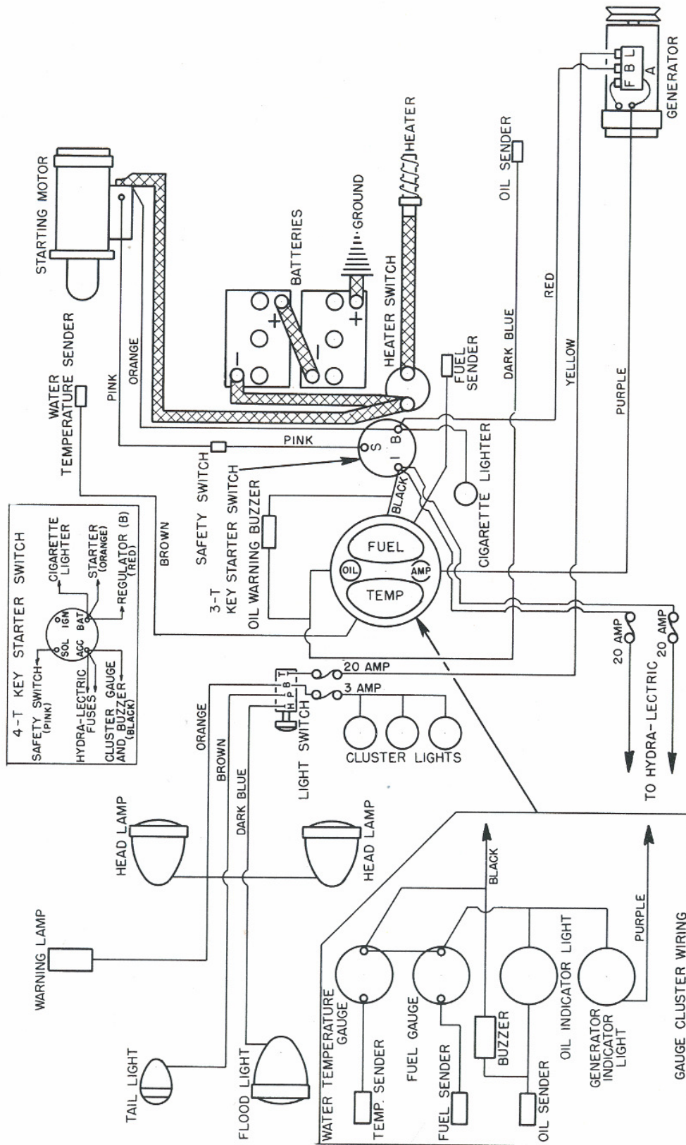
Figure 4-17 770, 880 Diesel 12-Volt Wiring Diagram
