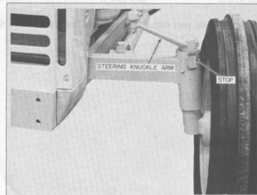
Figure 2 - Fixed Tread Axle With Superseded Steering Stop
