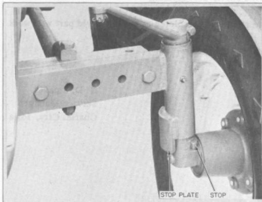
Figure 1 - Adjustable Front Axle With Current Steering Stop
