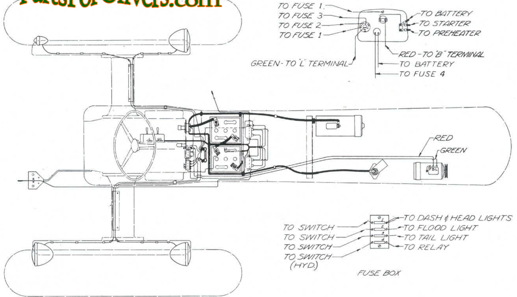
Figure 4-3 Fleetline 66, 77, 88 Diesel 12-Volt Wiring Diagram
